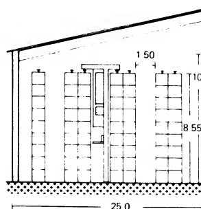
14 With stacker and extendable mast
